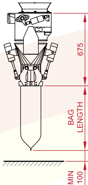
SYSTEM OVERALL DIMENSIONS
